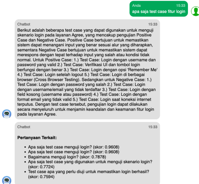
Gambar 4. 1 Eksperimen 1 Score Cosine Similarity
